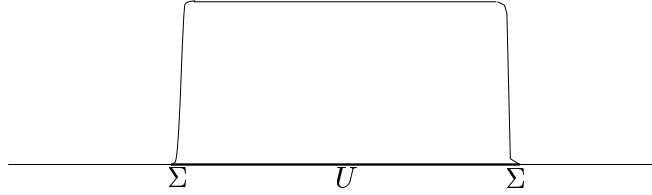
Figure 3: H_k
