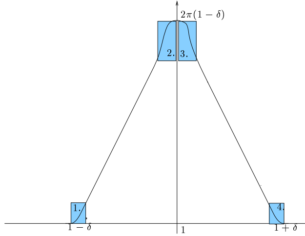
Figure 2: g_\delta , smoothened
