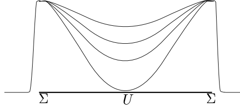
Figure 5: \tilde{H}_{k,s}
